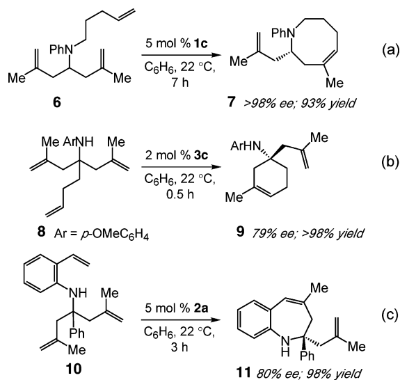
Scheme 1. Mo-Catalyzed ARCM of Unsaturated Arylamines
