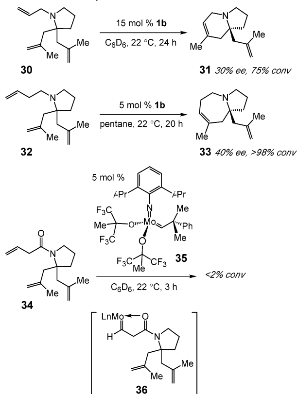
Scheme 5. Mo-Catalyzed ARCM of Amines and Isomeric Amides
