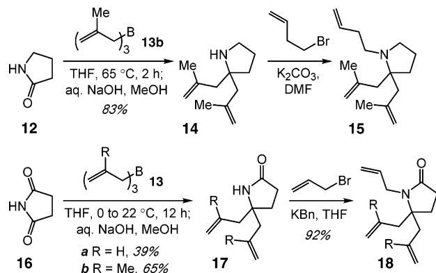
Scheme 3. Synthesis of Substrates for Mo-Catalyzed Enantioselective Synthesis of N-Fused Bicyclic Structures
