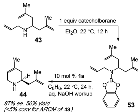
Scheme 6. Synthesis and Mo-Catalyzed ARCM of Catechol-Protected Amines
