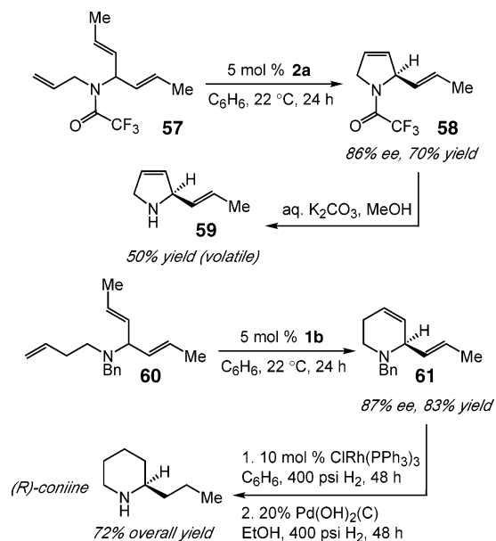
Scheme 8. Enantioselective Synthesis of Cyclic Amines Bearing Disubstituted Olefins
