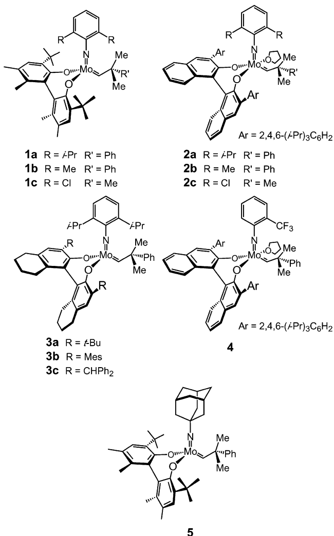
Scheme 1. Mo-Catalyzed ARCM of Unsaturated Arylamines
