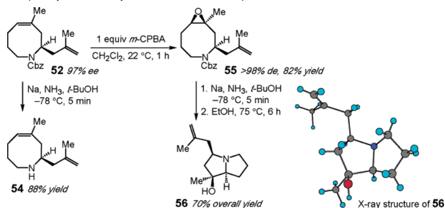
Scheme 8. Enantioselective Synthesis of Cyclic Amines Bearing Disubstituted Olefins
